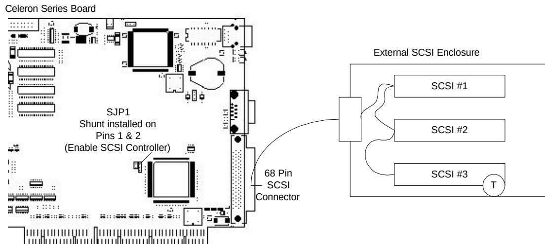
Figure 3 Configuration for Use of External SCSI Devices
